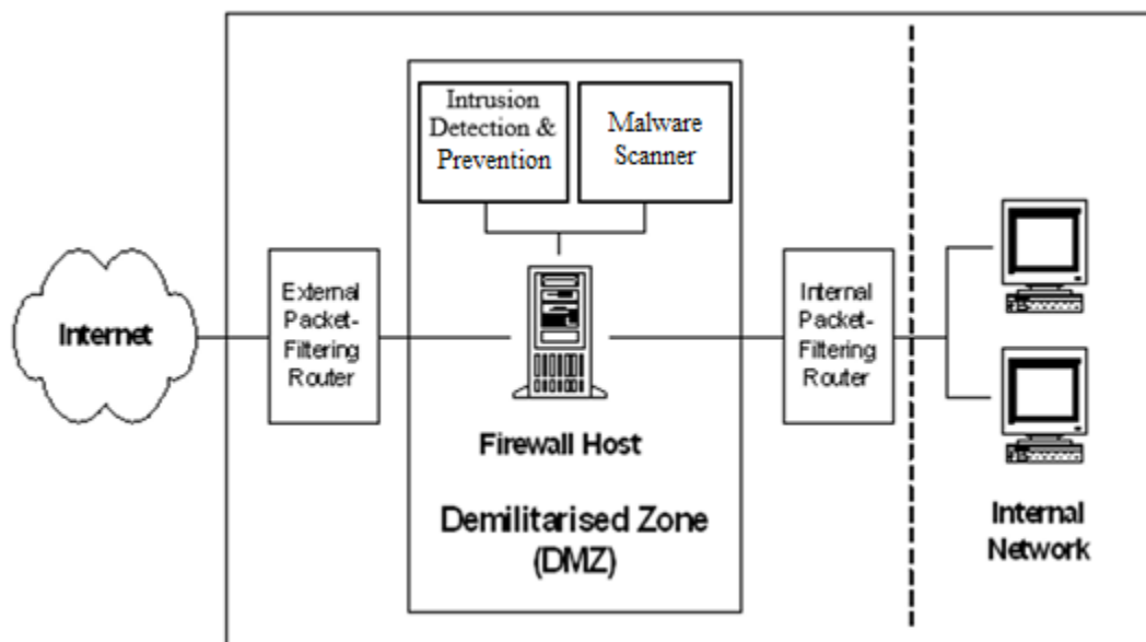
Figure 1 An Internet Gateway with Recommended Security Protection
